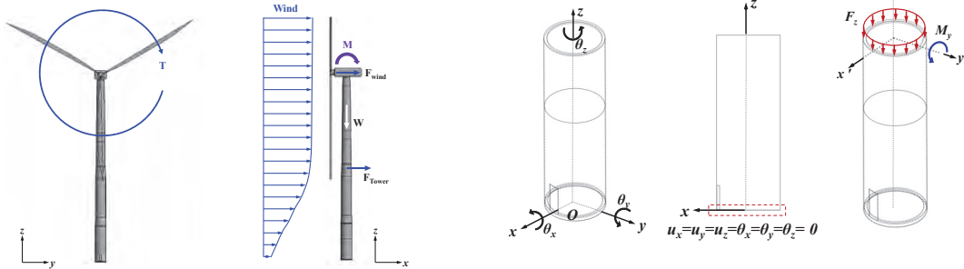
Fig. 8. Coordinate system and applied boundary conditions of the wind turbine tower: (a) coordinate system; (b) fixed boundary condition; (c) applied loading conditions.
