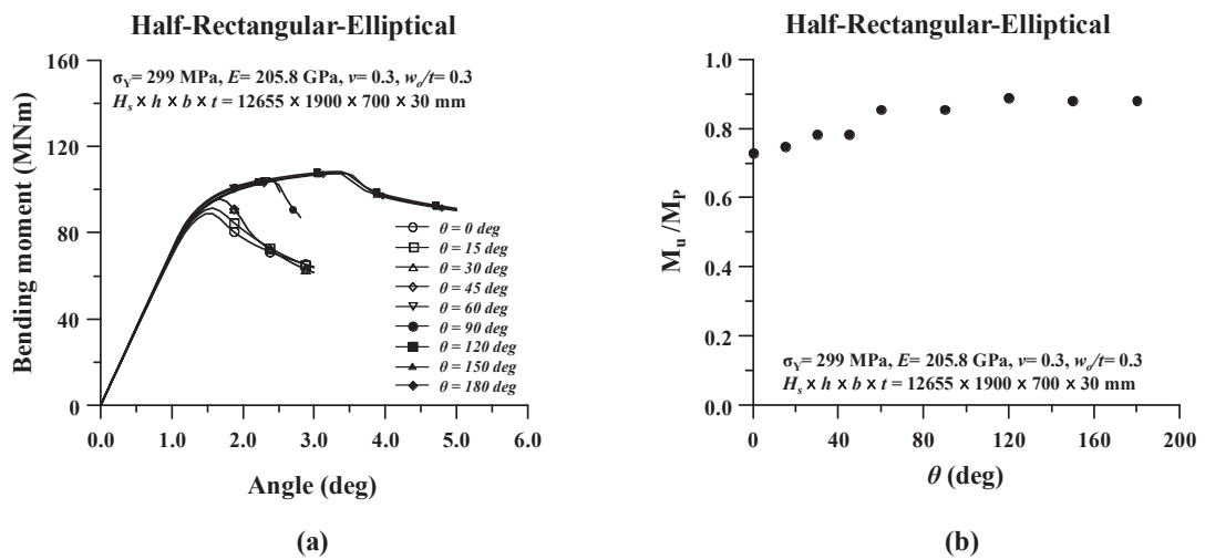
Fig. 19. Effect of cutout's angle under pure bending: (a) moment-rotation histories; (b) non-dimensionalized load carrying strength.
