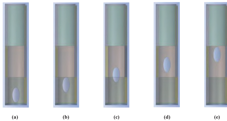
Fig. 14. An example of applied geometries with varying cutout's location in vertical direction: (a) h_o / H_S = 0.1 ; (b) h_o / H_S = 0.2 ; (c) h_o / H_S = 0.3 ; (d) h_o / H_S = 0.4 ; (e) h_o / H_S = 0.5 .
