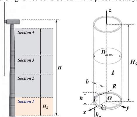
Fig. 4. Schematic representation of applied geometries.
