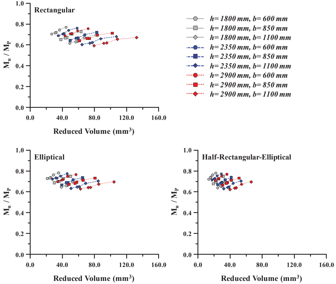
Fig. 21. An example of effect of column slenderness ratio for D_{\max} = 3750 mm under pure bending.
